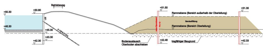
Bauphase I (Rammebene + neue Spundwand)
